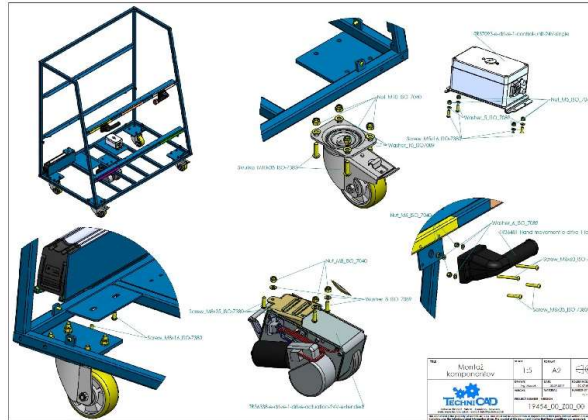
2D design
