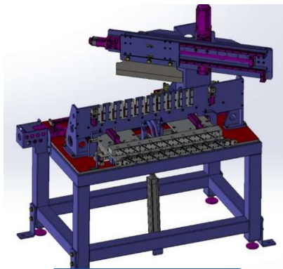
3D design
